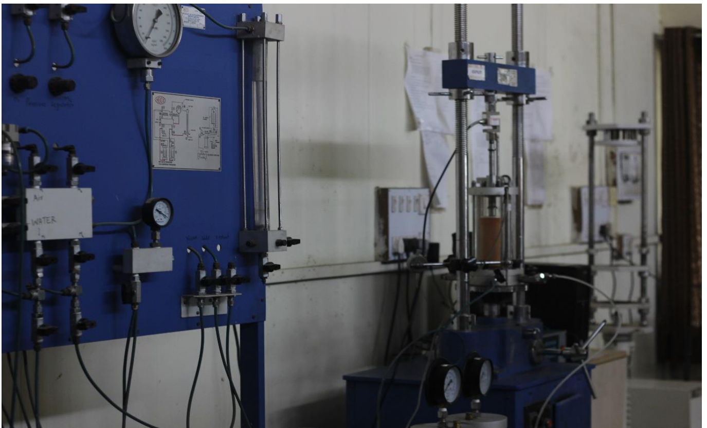
Triaxial Test Apparatus
