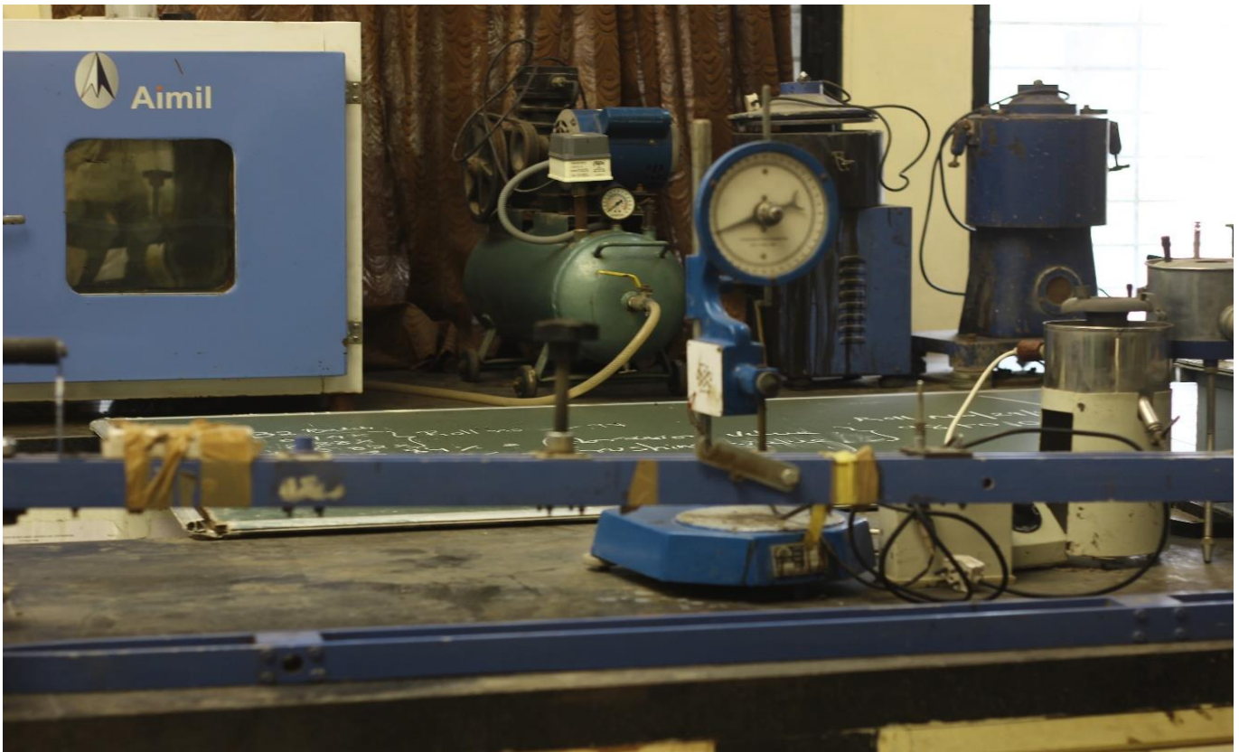
Rolling Thin Film Oven, Bitumen Extractor, Softening Point, Flash & Fire Point of Bitumen and Benkleman Beam Apparatus
